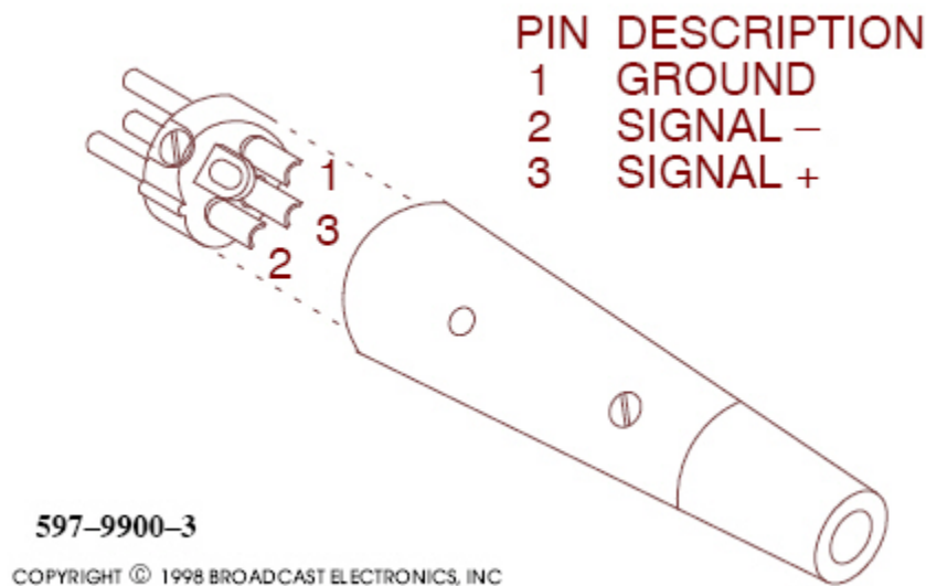
FIGURE 2. XLR PIN DESCRIPTIONS
